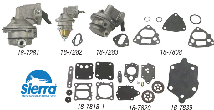
Fuel Pumps
